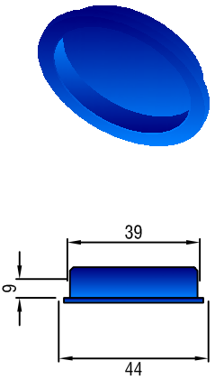
265P FINGER PULL - Plastic
