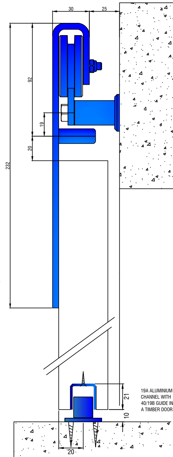
SECTION THROUGH DOOR SHOWING 30mm BAR TRACK WITH BRACKETS AND BARNSLIDE 50 HANGER. SCALE 1:2
