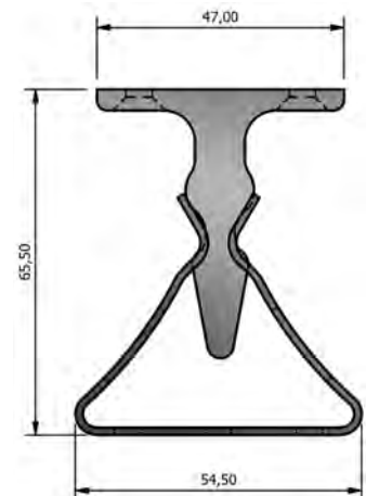
Vistafold® Hold Back Catch (SS)
