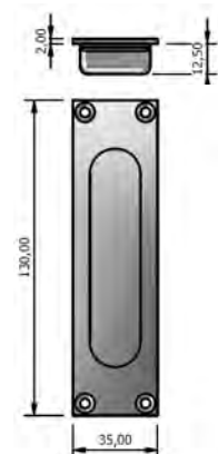
503SL Flush Pull Handle
