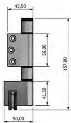
871x3 Meeting End Roller (RH)
