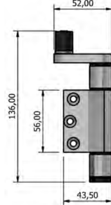
871x7 Meeting End Guide (RH)
