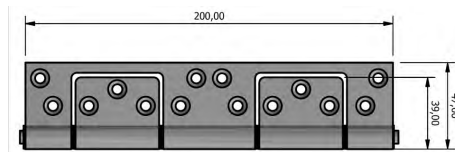
420 Sinkless Hinge (200mm)
