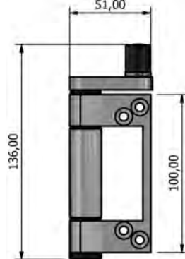
871x7 Meeting End Guide (LH)
