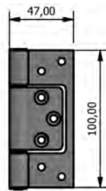
443 Sinkless Hinge (100mm)
