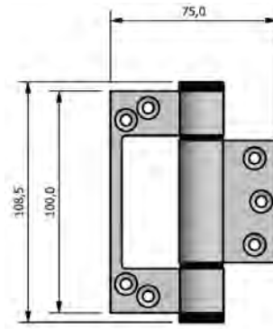
868x1 Sinkless Intermediate Hinge
