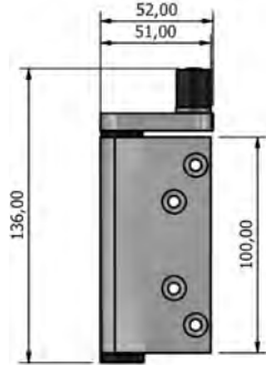
871x5 Full End Guide LH/RH
