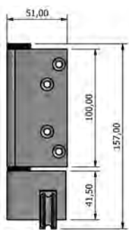
871x2 Full End Roller LH/RH
