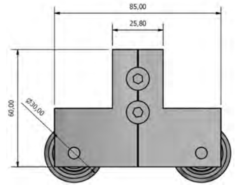
Vistafold® Mullion Roller
