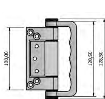
871 VSK Hinge Handle
