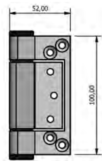
871x1 Cranked Hinge
