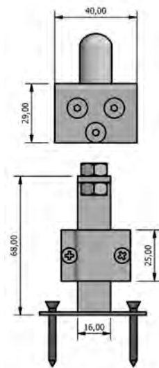
Flat/Round Shoot Kit
